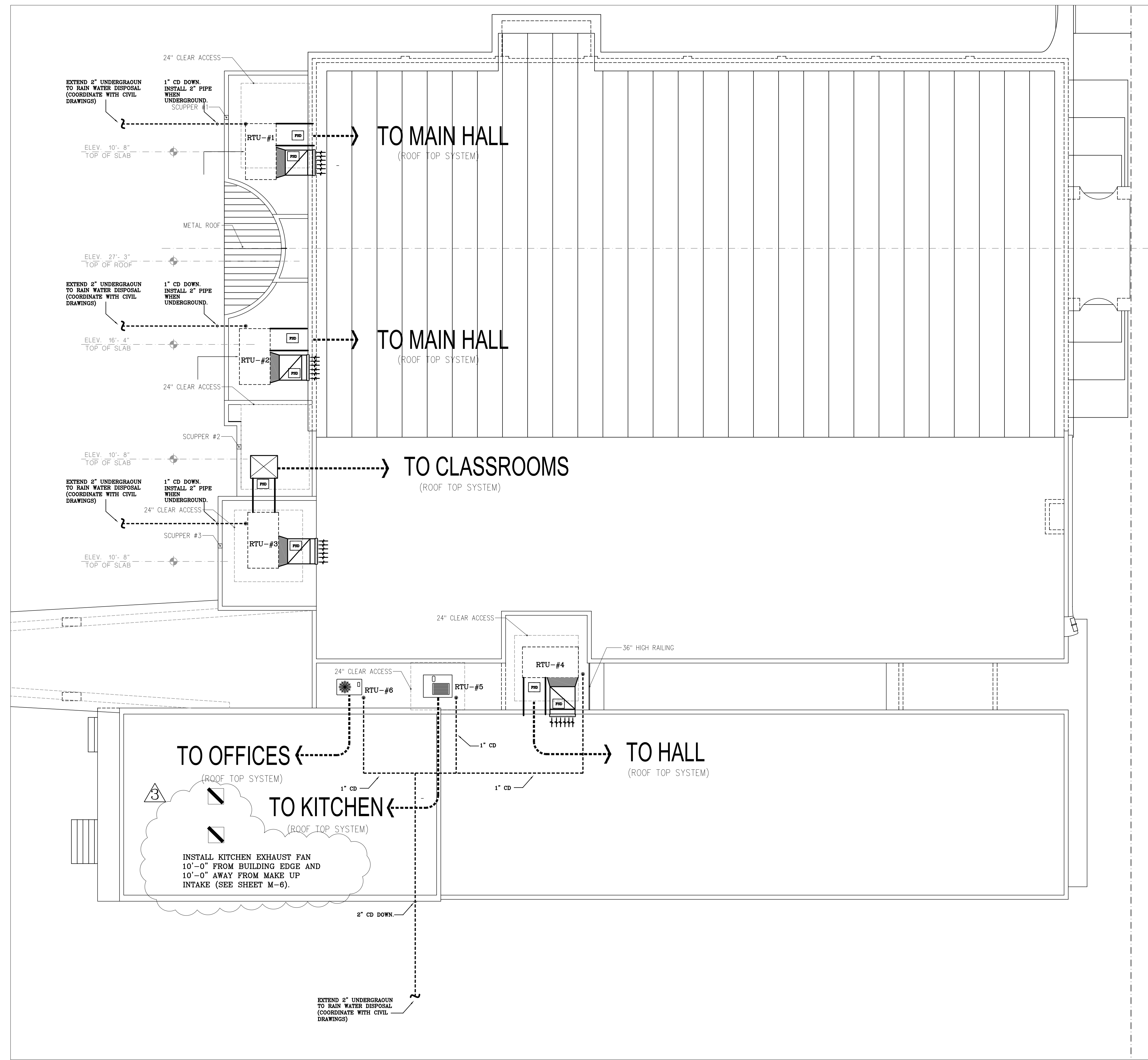
MECHANICAL ROOF PLAN SCALE: 1/8" = 1'-0"
