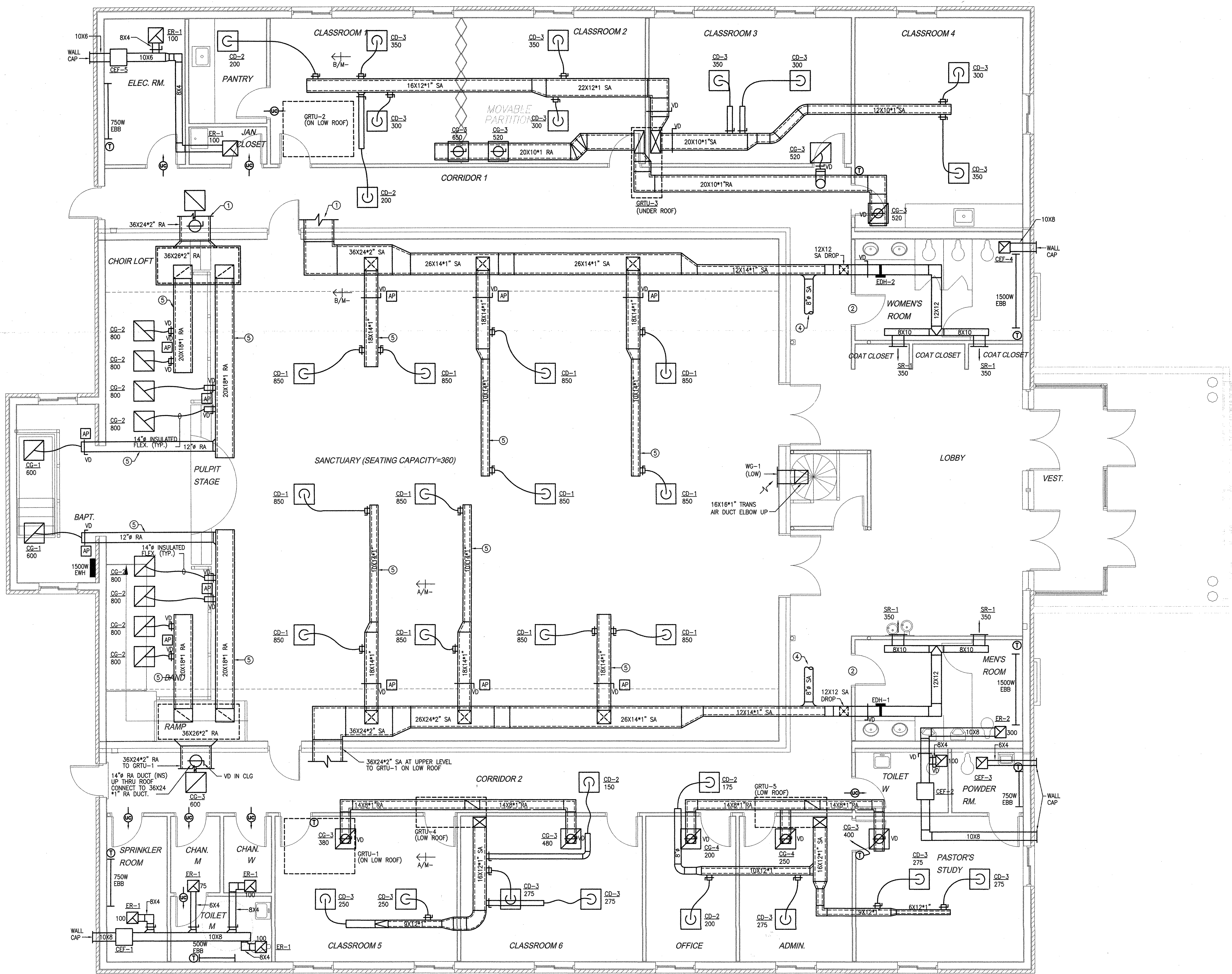
MECHANICAL PLAN (MEZZANINE) SCALE: 1/4" = 1'-0"
