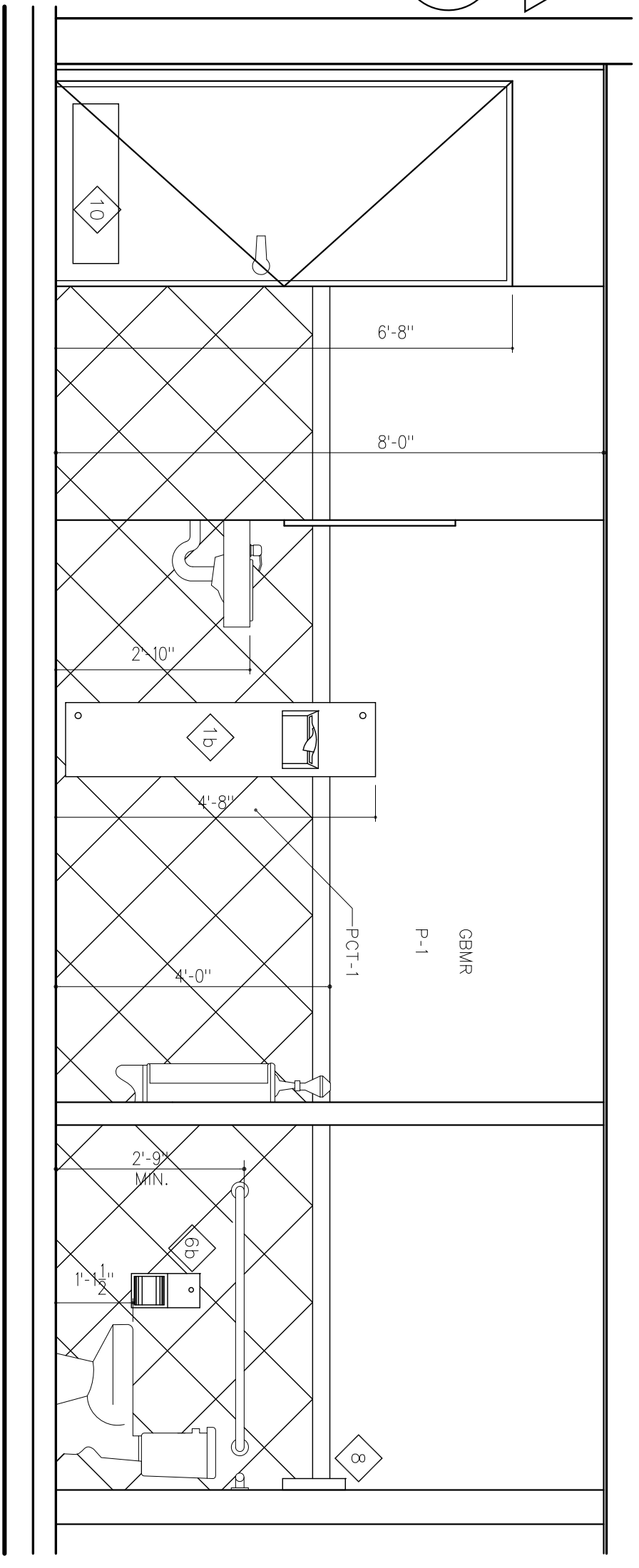
1 MEN RESTROOM ELEVATION BUILD. 2 SCALE: 1/2" = 1'-0"
