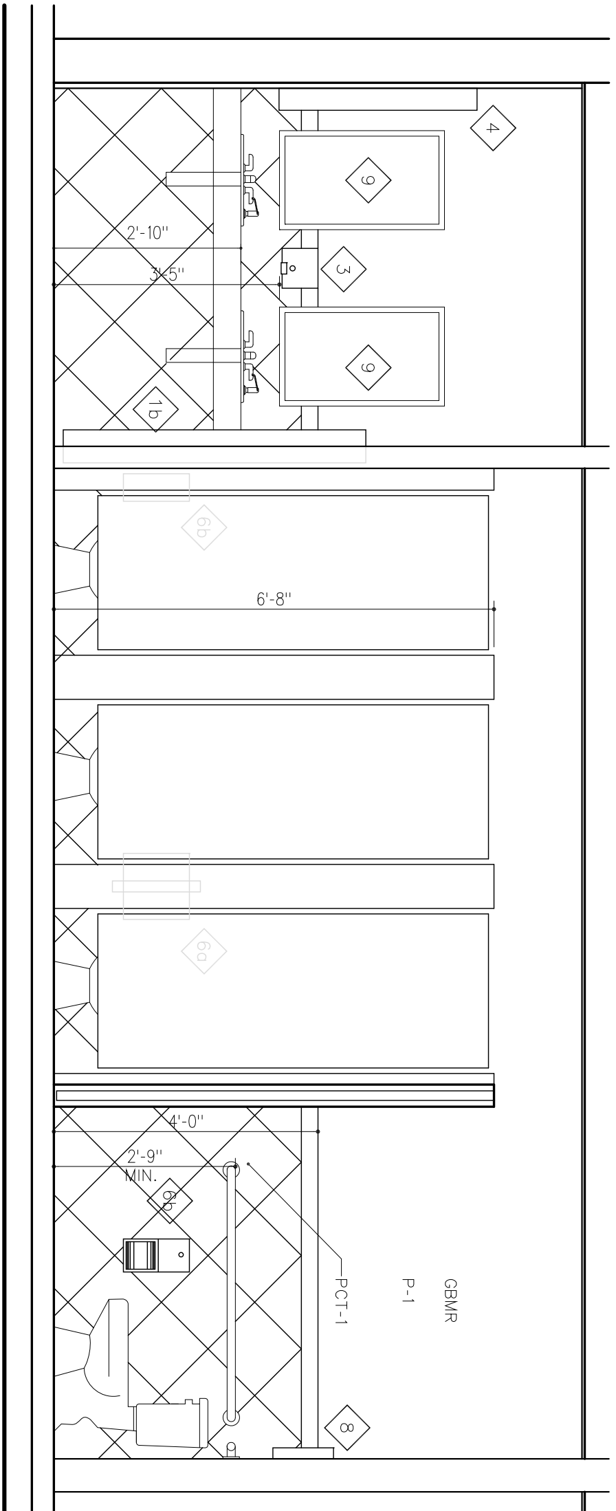
2 WOMEN BATHROOM ELEVATION BUILD. 2 SCALE: 1/2" = 1'-0"
